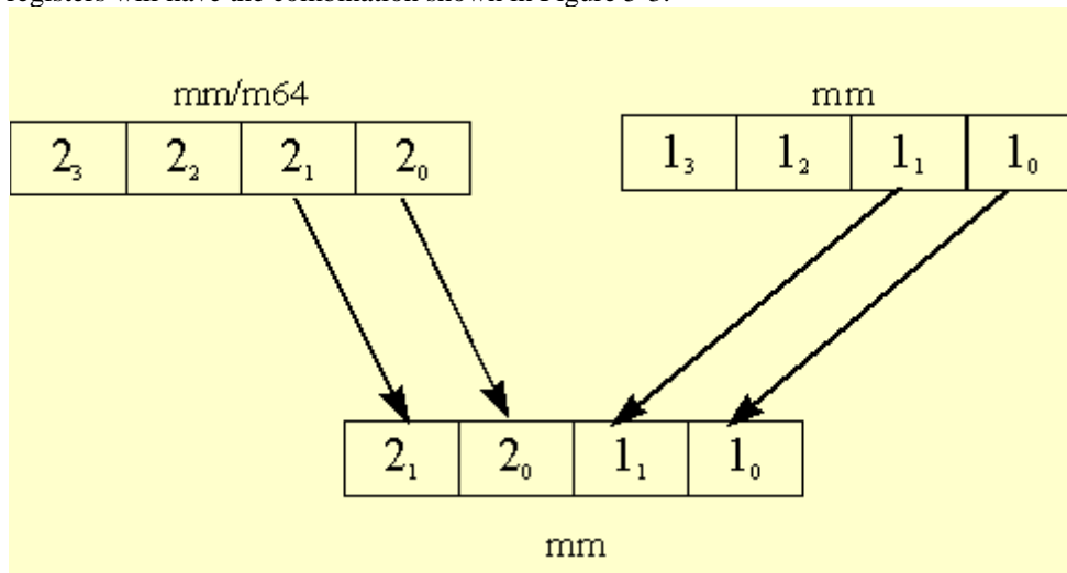
Figure 5-3. Result of Non-Interleaved Unpack in MM0
