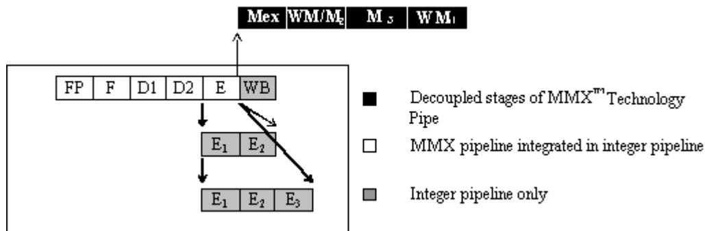
Figure 2-1. MMX™ Technology Pipeline Structure
