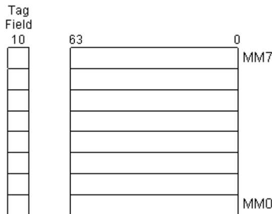
Figure 1-2. MMX™ Register Set
