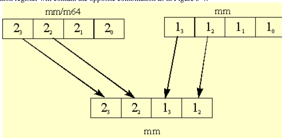
Figure 5-4. Result of Non-Interleaved Unpack in MM1
