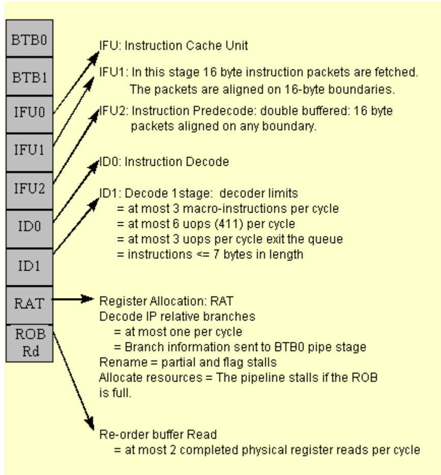
Figure 2-3. Out-Of-Order Core and Retirement Pipeline
