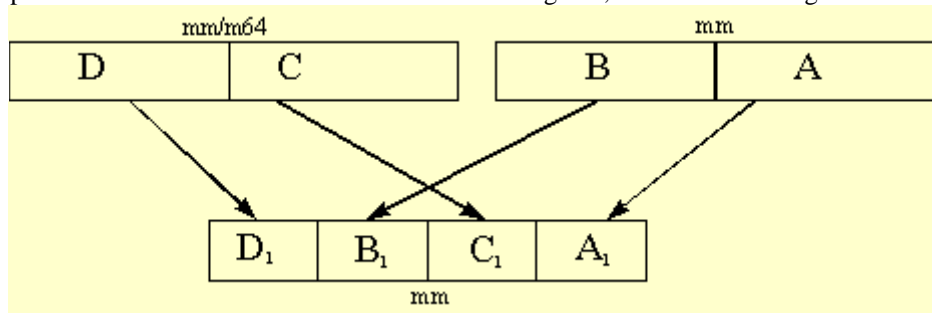
Figure 5-2. Interleaved Pack with Saturation Example
