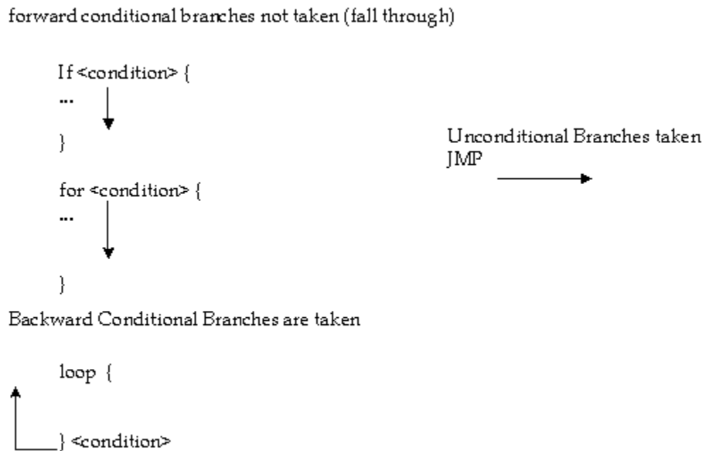
Figure 3-2. Dynamic Execution (P6-Family) Static Branch Prediction Algorithm
