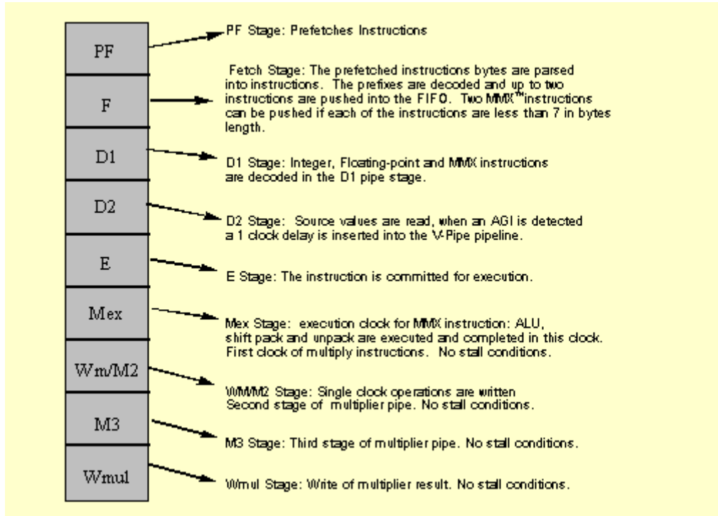
Figure 2-2. MMX™ Technology Instruction Flow in a Pentium® Family Processor with MMX Technology
