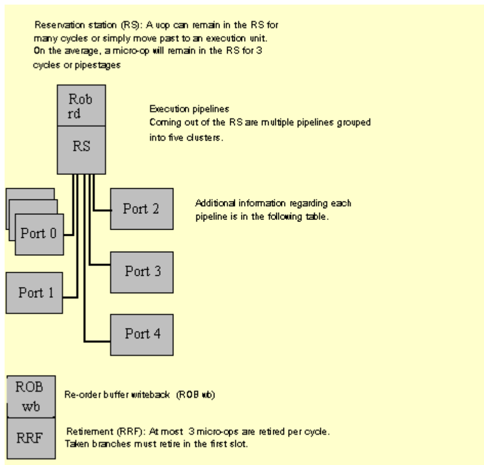
Figure 2-4. Out-Of-Order Core and Retirement Pipeline
