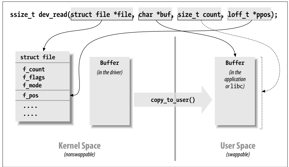
Figure 3-2. The arguments to read
